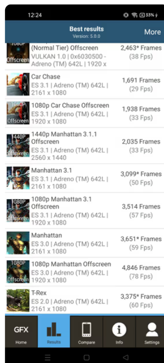
Graphics Benchmark
