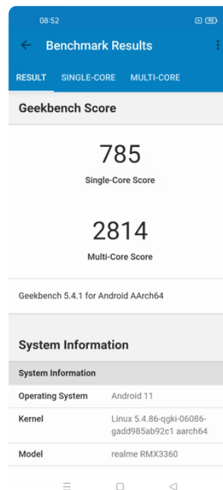
GeekBench5 Benchmark
