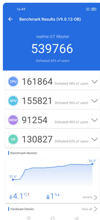
AnTuTu Benchmark
